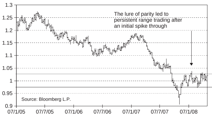
Figure 7.4 USDCAD weekly
