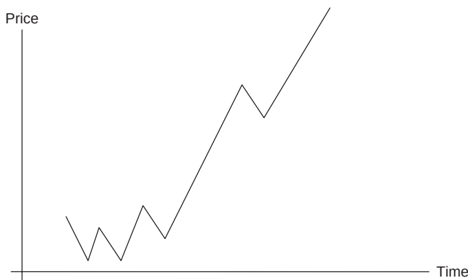
Figure 3.4 Volatility
