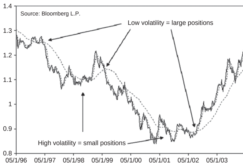
Figure 23.2 EURUSD weekly
