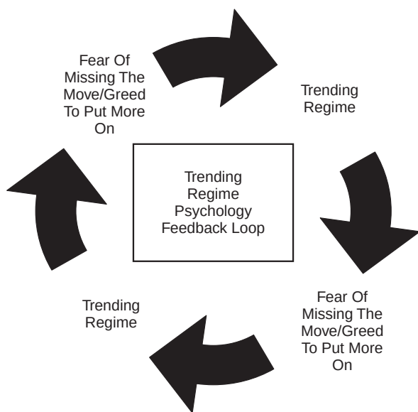
Figure 3.18 Trending Regime
